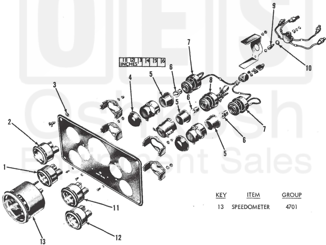
Figure 32. Instrument panel
